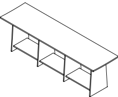
Panca/Bench L 140 P 38 H 42 cm
